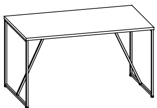
LST 1380 1360x800x750
